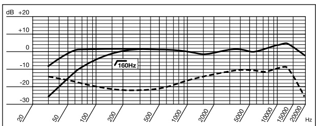
Frequency Response
