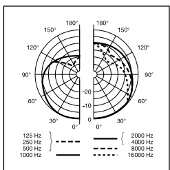
Polar Diagram
