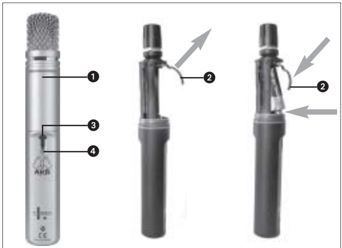
Fig. 1: Inserting a battery.
